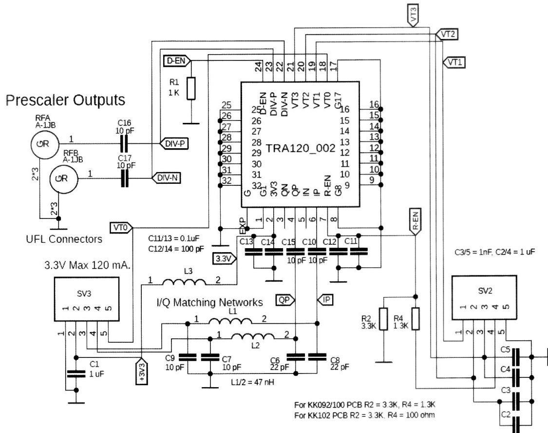
Fig. 8: 122 GHz transceiver module, RF PCB circuit diagram
