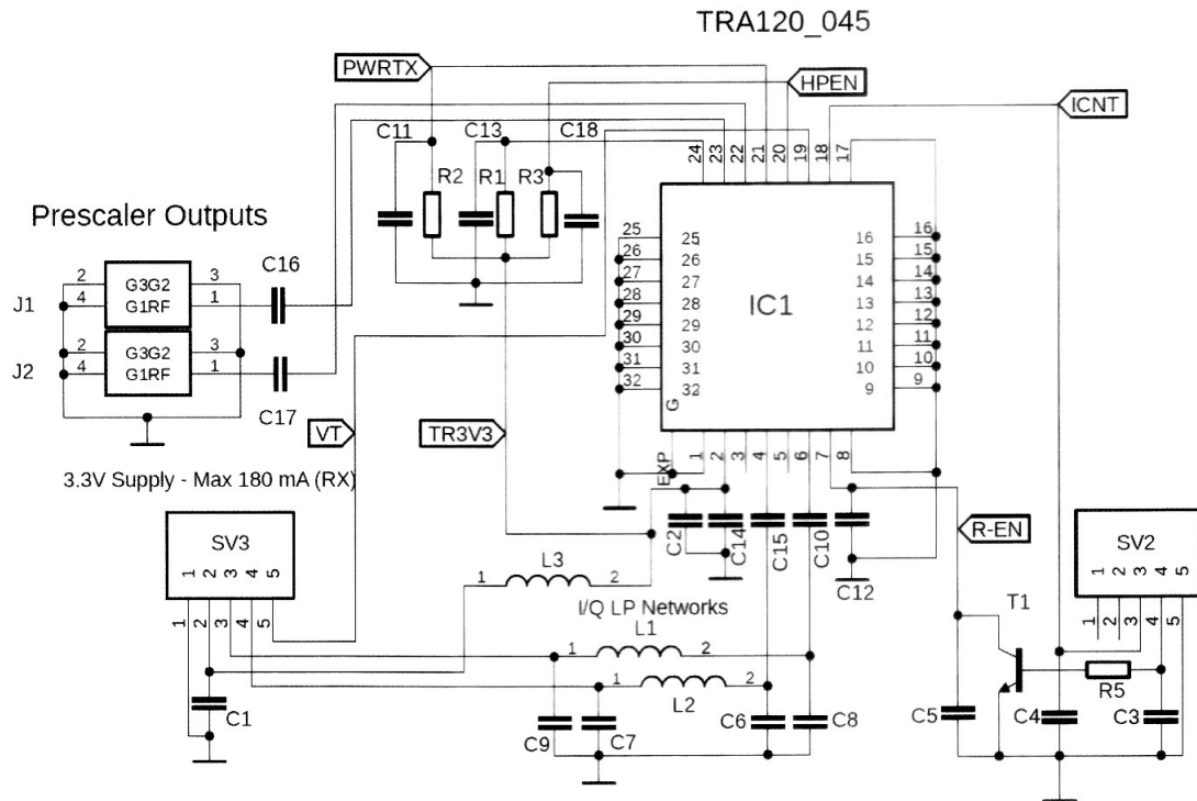
Fig. 9: 122/134 GHz transceiver module, RF PCB circuit diagram
